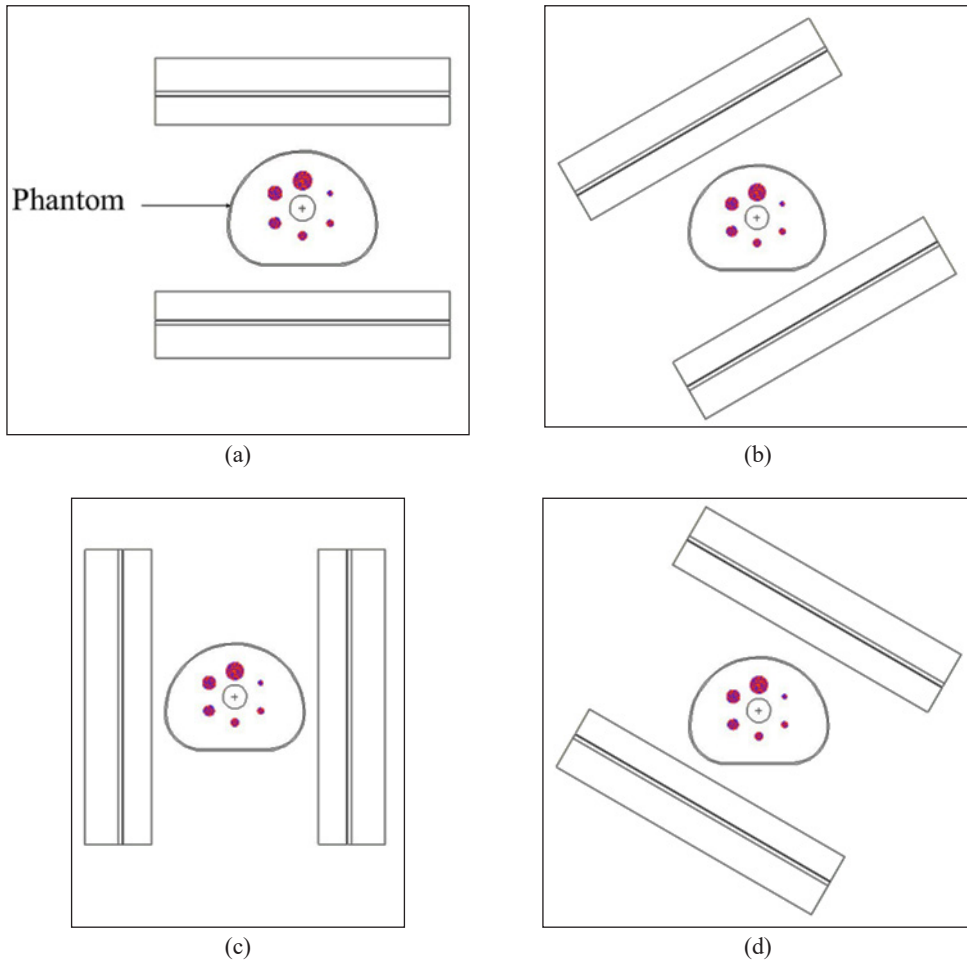
Figure 3. The geometry of the NEMA phantom and simulated SPECT system, as viewed in VisEd, is shown at different rotation angles: (a) 0°, (b) 30°, (c) 90°, and (d) 150°, with a clockwise rotation
